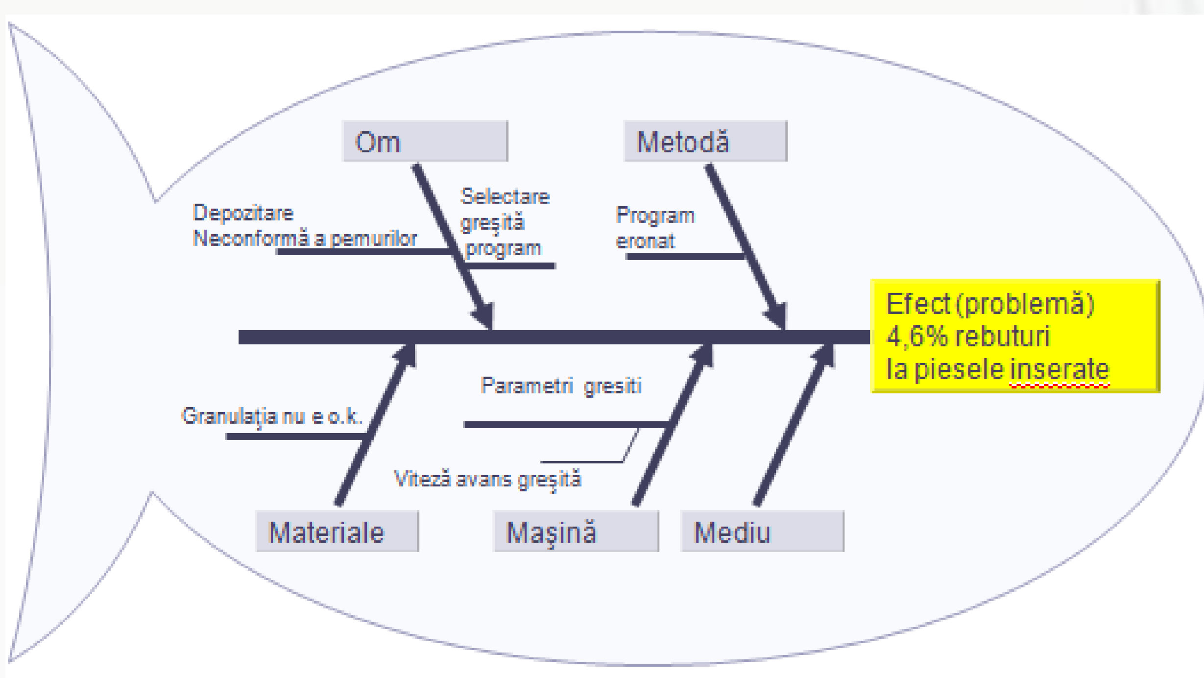
Fig.3. Diagrama Cauza – Efect Ishikawa
